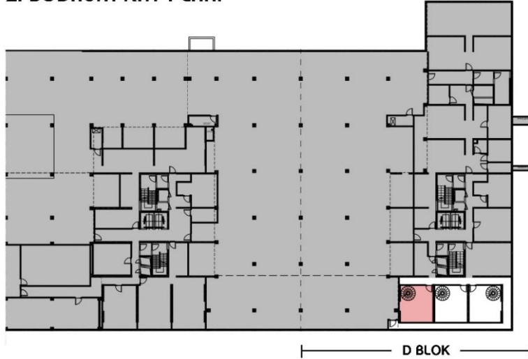
2. BODRUM KAT PLANI
